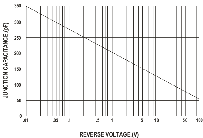
FIG.4-TYPICAL JUNCTION CAPACITANCE
